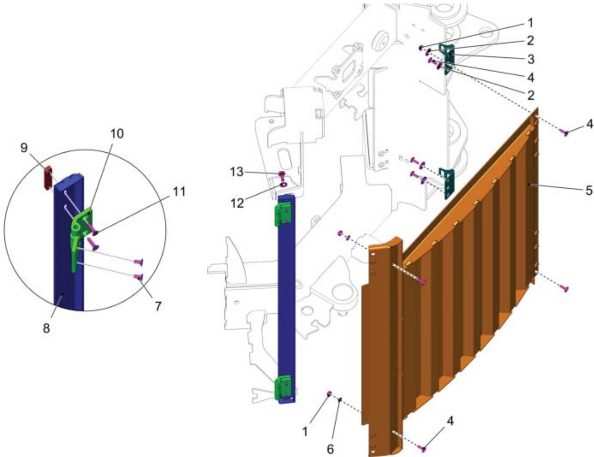
PARTS LIST - MOUNTING MATERIAL COOLING RIGHT
