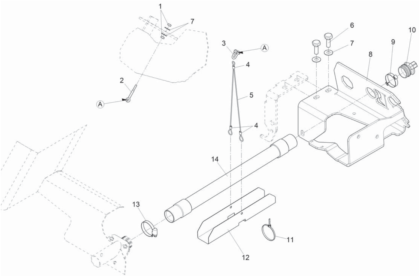
PARTS LIST - HOSE - BRACKET
