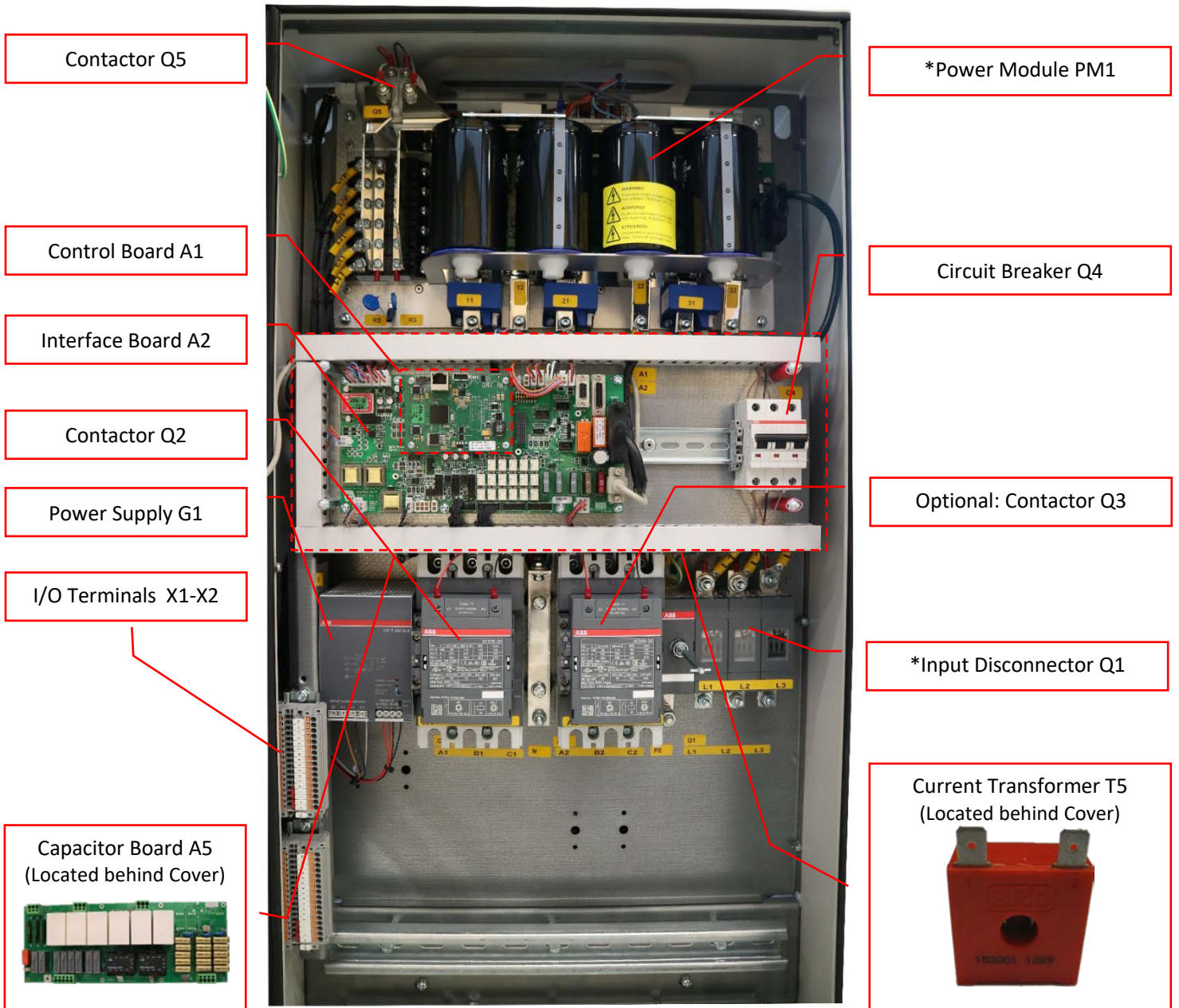
Figure 5: Front View Internal Components
