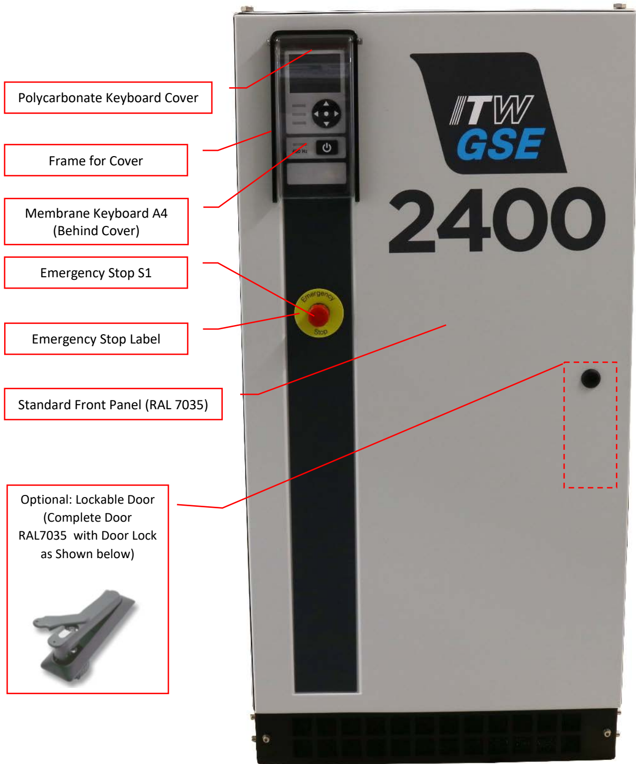
Figure 1: Front View
