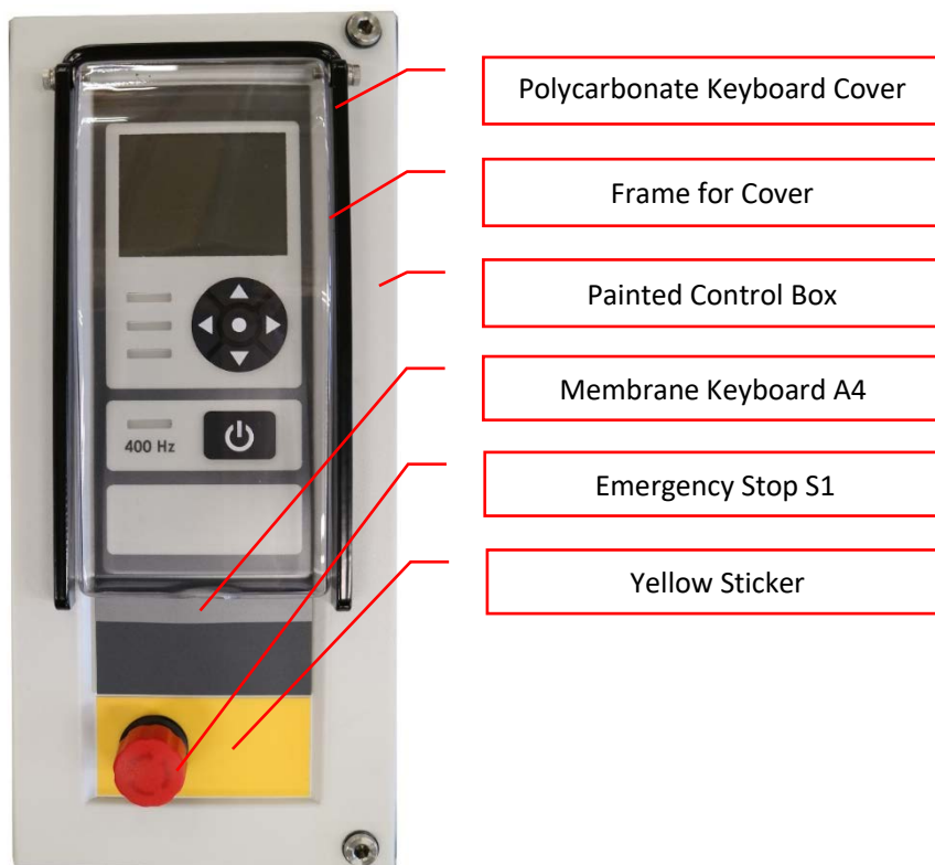
Figure 10: Front View Remote Control Box
