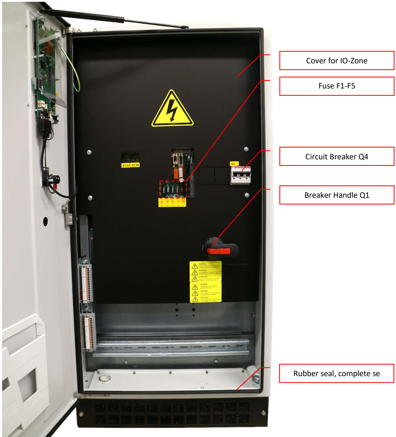
Figure 4: Front Cover Internal
